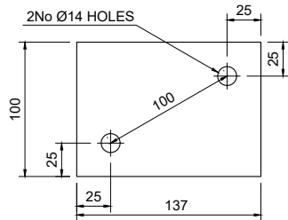
TPL-1 - 10mm THICK Scale 1:5
