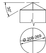
DETAIL A - TIMBER POLE TOP Scale 1:20
