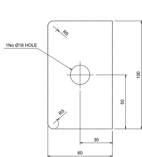
TPC-A-1 - 15mm THICK Scale 1:2
