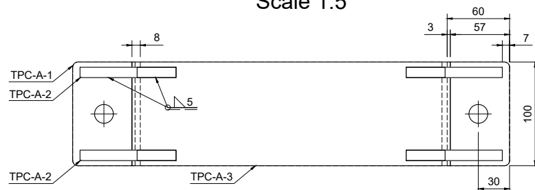
TPC-A Scale 1:5
