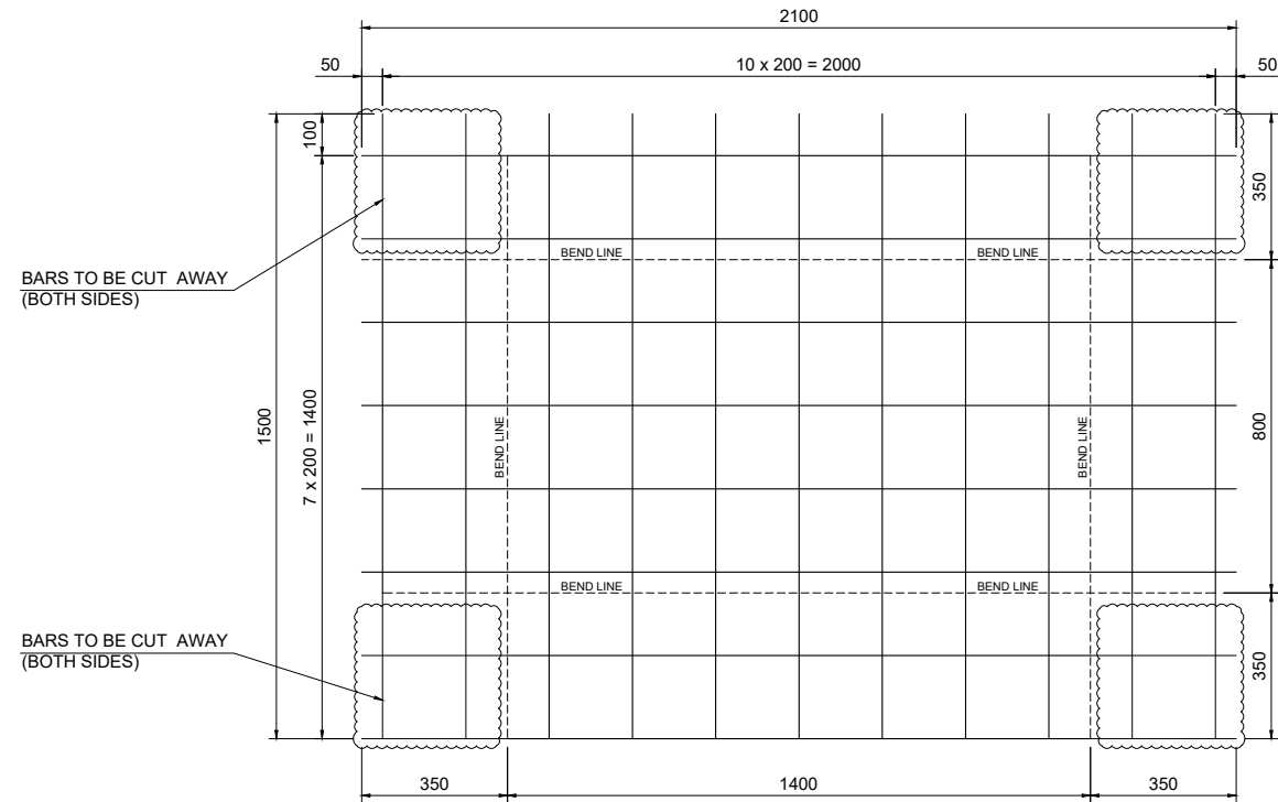
01- A252 MESH 1500x2100mm Scale 1:20
