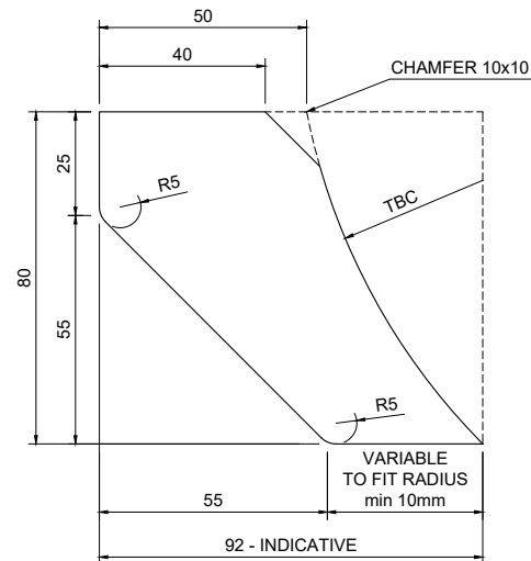
TPC-A-2 - 10mm THICK Scale 1:2
