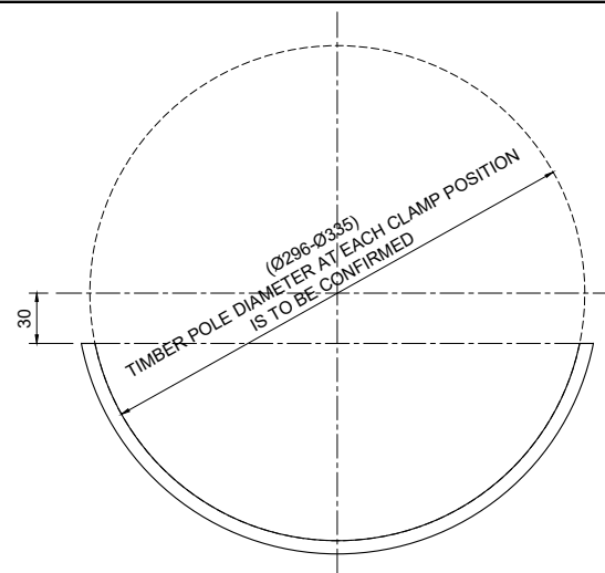
TPC-A-3 - 100x8mm PLATE Scale 1:5
