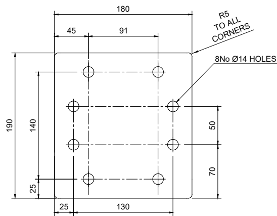
TPB-B-5 - 10mm THICK Scale 1:5
