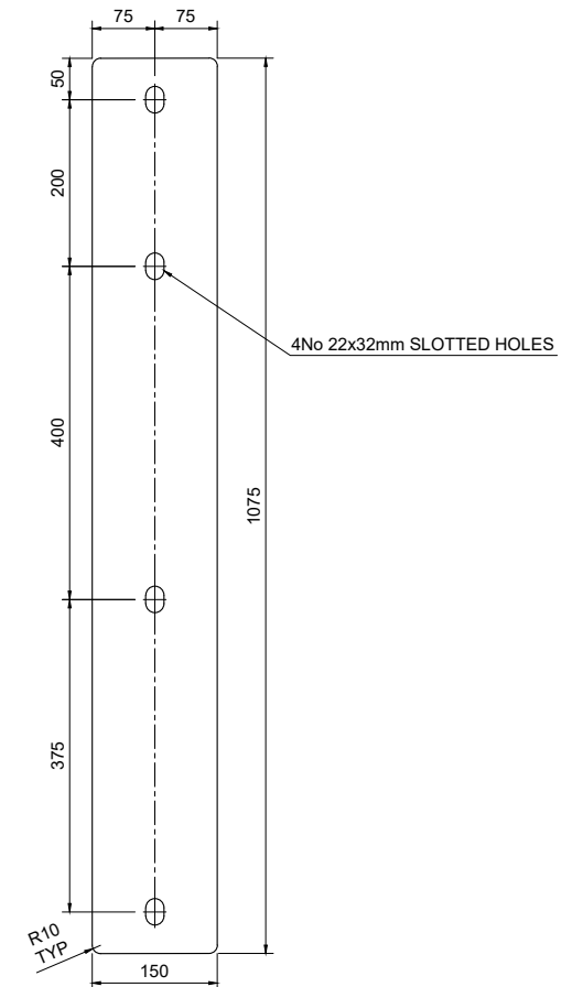
TPC-B - 15mm THICK Scale 1:10
