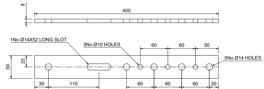
TPA-PD - 8mm THICK Scale 1:5
