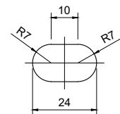
SLOTTED HOLE DETAIL Scale 1:2
